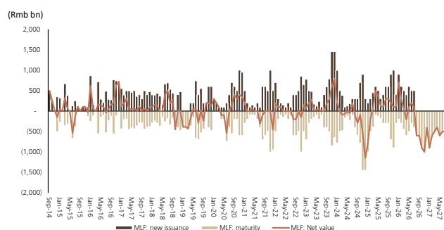
Figure 10: MLF
